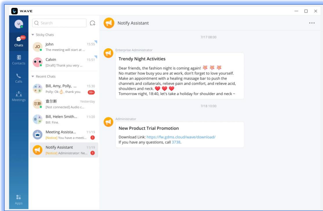
Figure 11: Notification Assistant
