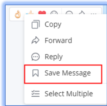
Figure 2 - Save Message
